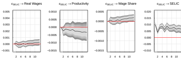
Figure 11: Impulse Response Functions (IRFs), Model 1 (Alternative Ordering - Taylor Rule): Figures display IRFs of Real Wages, Productivity, Wage Share, and SELIC to monetary policy (SELIC) shocks. Quarters on x-axis. Shaded grey areas denote 95%, 90%, 84% and 68% confidence bands calculated through m.b. bootstrapping (1000 runs).
