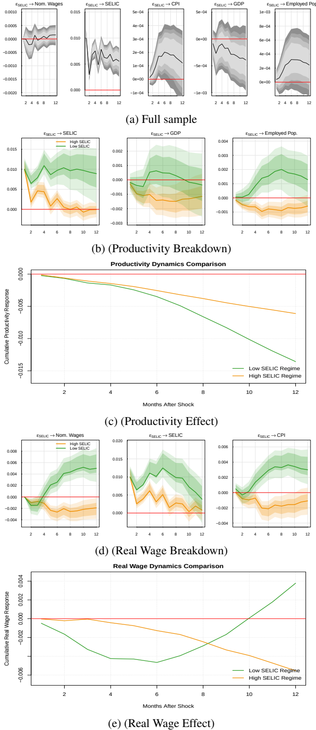
Figure 4: Impulse Response Functions (IRFs), Model 2: Figures display IRFs of SELIC, Nominal Wages, CPI, GDP, and Employed Population to monetary policy (SELIC) shocks. Shaded grey areas denote 95%, 90%, 84% and 68% confidence bands calculated through m.b. bootstrapping (1000 runs). Panels (4b)-(4d) further decompose productivity and real wages into their respective components. Results are presented for two regimes: low interest rate (green) and high interest rate (yellow). Shaded green and yellow areas denote 90% and 68% confidence bands calculated through m.b. bootstrapping (1000 runs).
