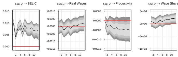
Figure 3: Impulse Response Functions (IRFs), Model 1: Figures display IRFs of SELIC, Real Wages, Productivity, and Wage Share to monetary policy (SELIC) shocks. Quarters on x-axis. Shaded grey areas denote 95%, 90%, 84% and 68% confidence bands calculated through m.b. bootstrapping (1000 runs).
